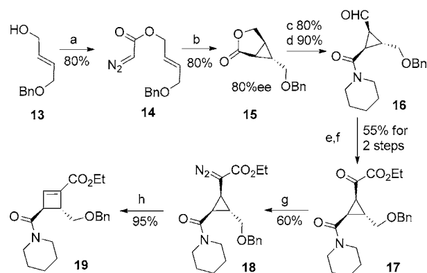
Scheme 2. Stereoselective synthesis of cyclobutenolate. Reagents and conditions: a) Bromoacetyl bromide then TsNHNHTs, DBU. b) 1.0 mol % [\text{Rh}_2(5\text{S-MEPY})_4] , \text{CH}_2\text{Cl}_2 , reflux. c) piperidine, \text{AlMe}_3 , \text{CH}_2\text{Cl}_2 , 0°C to RT, 20 h. d) DMSO, (\text{COCl})_2 , \text{Et}_3\text{N} , –78°C, 2 h. e) NaCN, HOAc, MeOH then EtOH/HCl (4 M in 1,4-dioxane) (1:1), 0°C, 2 days. f) Dess–Martin periodinane, \text{CH}_2\text{Cl}_2 , RT, 2 h. g) TsNHNHTs, toluene, 80°C, then DBU, RT, 12 h. h) 10 mol % AgOTf, \text{CH}_2\text{Cl}_2 , RT, 2 h. Bn = benzyl, DBU = 1,8-diazabicyclo[5.4.0]undec-7-ene, MEPY = methyl-2-pyrrolidone-5S-carboxylate.
