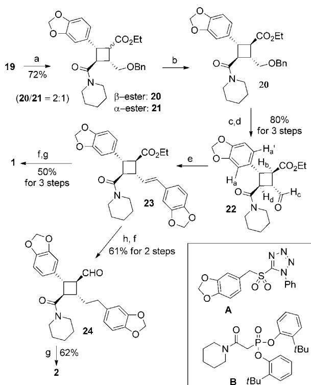
Scheme 3. Stereoselective synthesis of proposed structures of piper-cyclobutanamide A and piperchabamide G. Reagents and conditions: a) 5.0 mol % [\text{Rh}(\text{cod})\text{Cl}]_2 , 1,4-dioxane/ \text{H}_2\text{O} (10:1), 3,4-(methylenedioxy)phenylboronic acid, RT, 20 h. b) \text{EtONa} , \text{EtOH} , RT, 10 h. c) \text{Pd/C} , \text{H}_2 , \text{EtOH} , RT, 15 h. d) Dess–Martin periodinane, \text{CH}_2\text{Cl}_2 , RT, 2 h. e) KHMDS, reagent A, DMF/HMPA (3:1), -35^\circ\text{C} to RT, 6 h. f) DIBALH, toluene, -78^\circ\text{C} , 30 min. g) KHMDS, reagent B, THF -78^\circ\text{C} to 0^\circ\text{C} , 2 h. h) \text{Pd/C} , \text{H}_2 , \text{MeOH} , RT, 15 h. cod = 1,5-cyclo-octadiene, DIBALH = diisobutylaluminum hydride, DMF = N,N' -dimethylformamide, HMPA = hexamethylphosphoramide, KHMDS = potassium hexamethyldisilazide.
