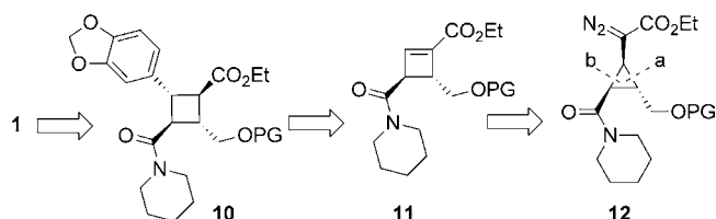
Scheme 1. Proposed strategy for stereoselective synthesis of pipericyclobutanamide 1 and piperchabamide 2 . PG = protecting group.
